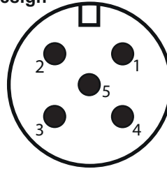
Pin Design
